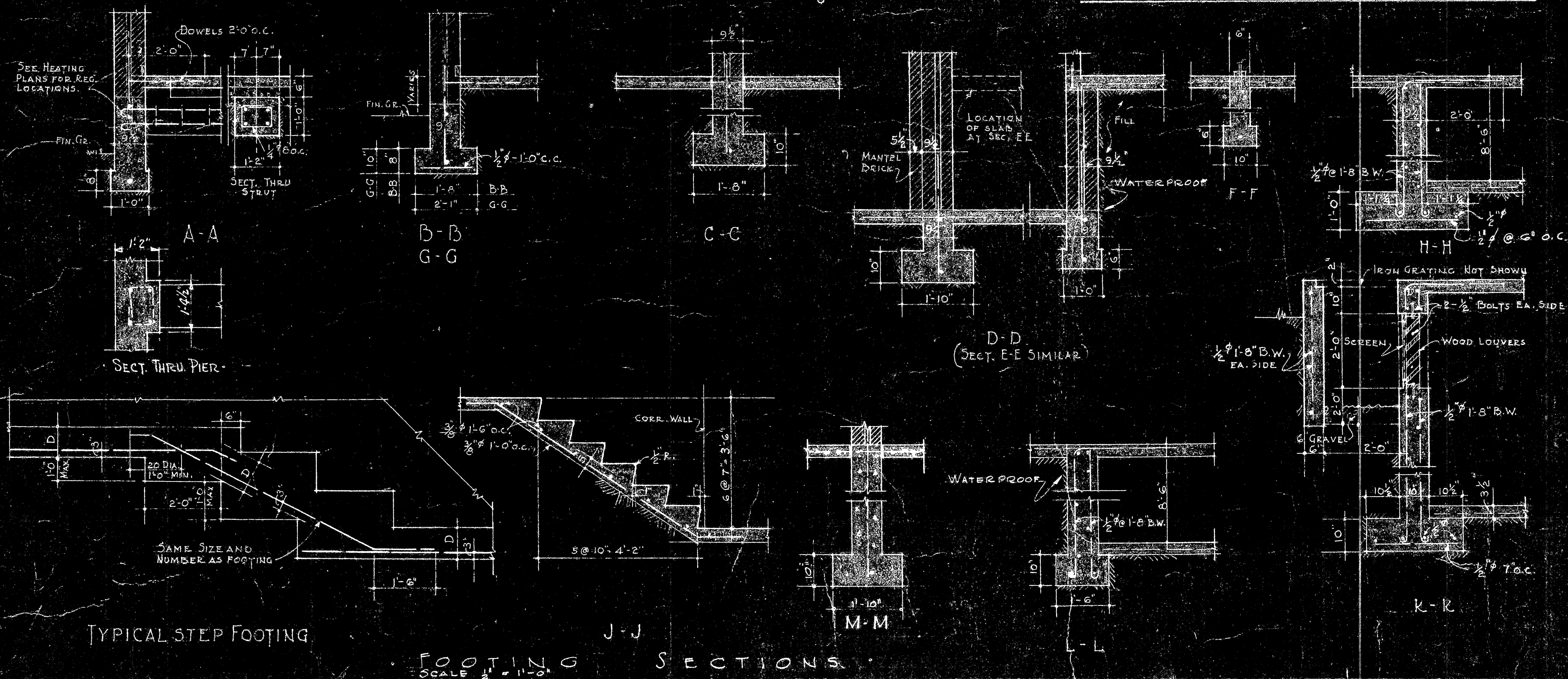
BASEMENT & FOOTINGS Scale 1/8" = 1'-0"
