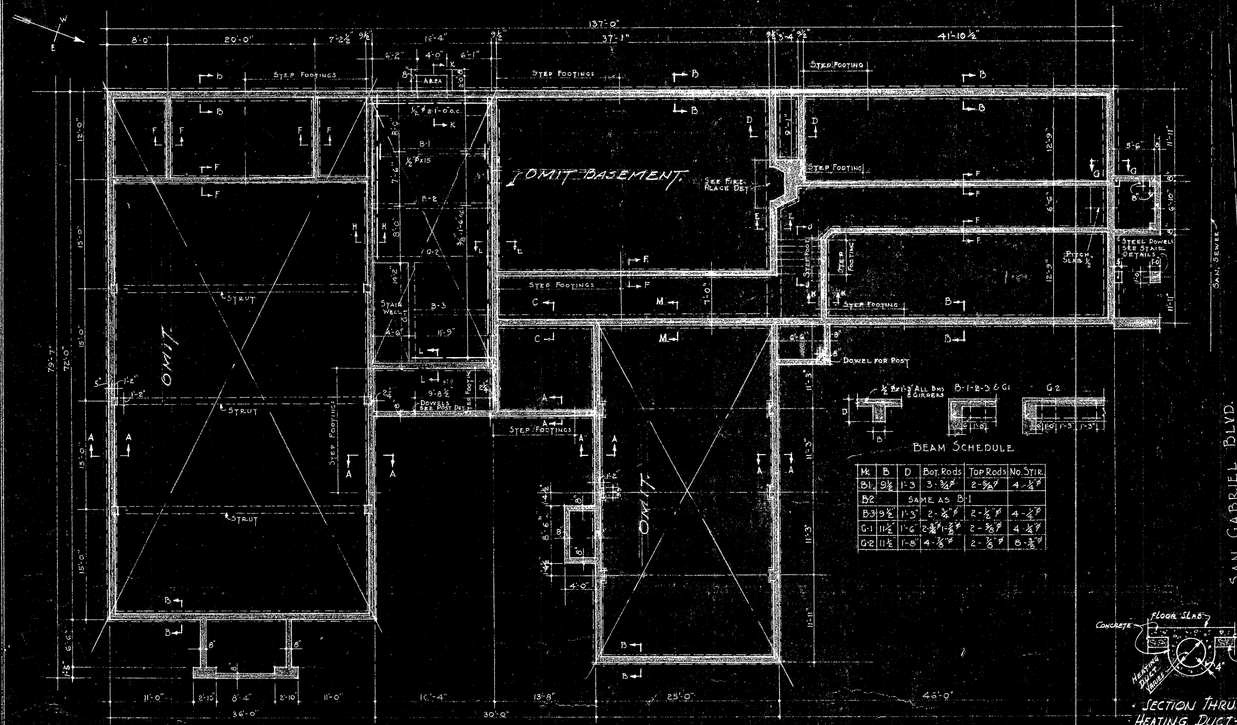
BASEMENT & FOOTINGS Scale 1/8" = 1'-0"
